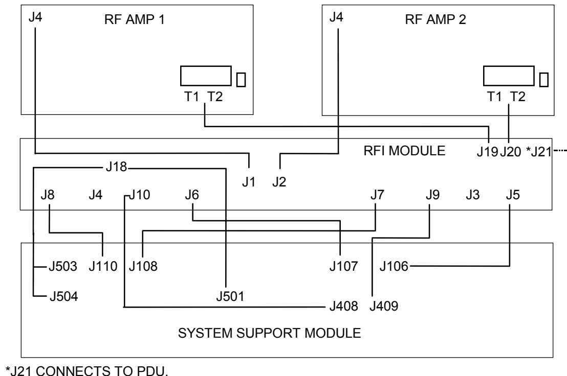
SSM REAR CABLE INTERCONNECTS ILLUSTRATION 1-1
