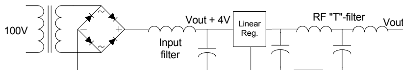
TYPICAL LINEAR REGULATOR CIRCUIT ILLUSTRATION 4-4
